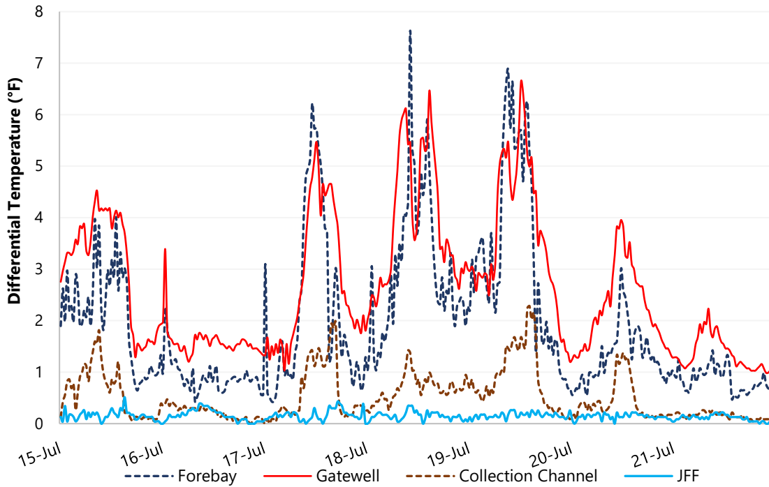
Figure 4 Average Differential Temperatures within Four Dam Locations from July 16 to July 22
