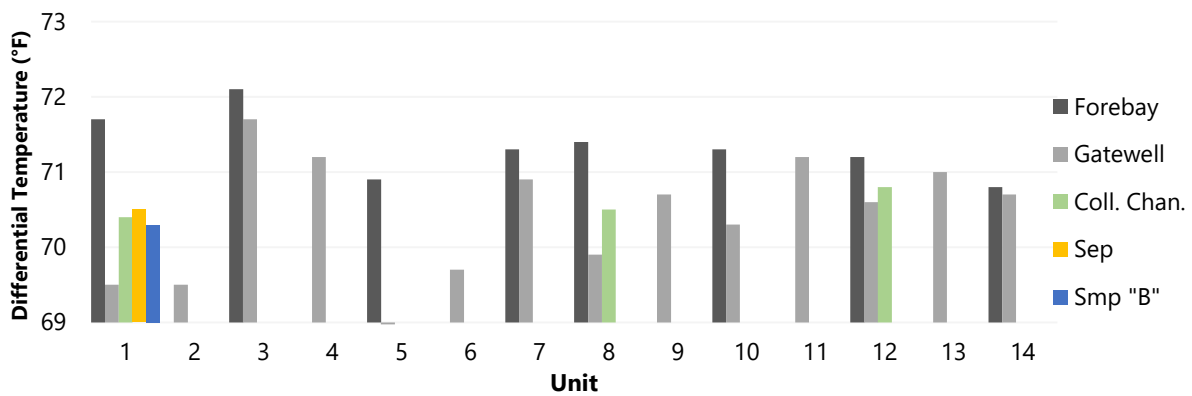
Figure 3 Average Weekly Water Temperatures by Position for Five Dam Locations from July 16 to July 22
