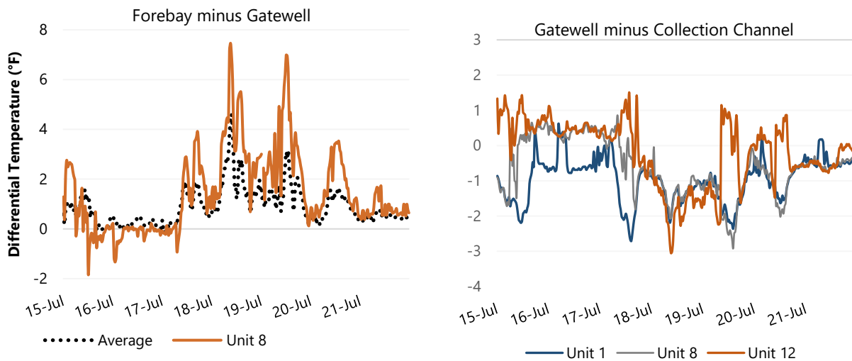
Figure 5 Average Differential Temperatures across Three Dam Locations from July 16 to July 22
