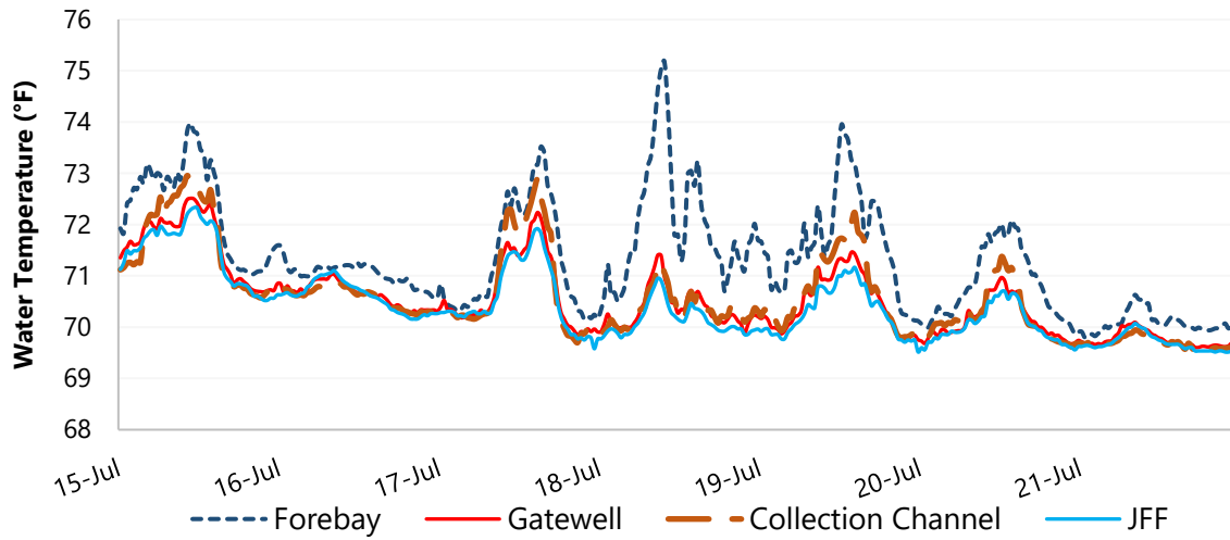
Figure 2 Average Water Temperatures for Each Half-Hour Interval for Four Dam Locations from July 16 to July 22
